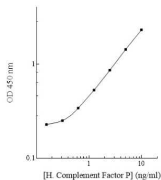
Human Complement Factor P Standard Curve
