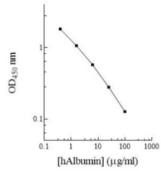
Albumin Calibration Curve
