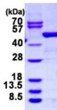
15% SDS-PAGE (3ug)
