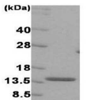
15% SDS-PAGE (3ug)
