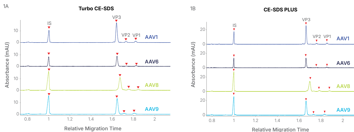
FIGURE 1. Identifying different AAV serotypes with Maurice CE-SDS. A. Stacked profiles of four different AAV serotypes analyzed with the Turbo CE-SDS cartridge and B. the Maurice CE-SDS PLUS cartridge. Both methods could easily distinguish between serotypes. The internal standard is labeled as IS.
