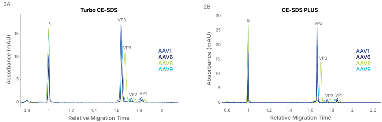
FIGURE 2. Overlaid profiles of the same four AAV serotypes analyzed with A. the Turbo CE-SDS cartridge and B. the Maurice CE-SDS PLUS cartridge show the differences between serotypes.
