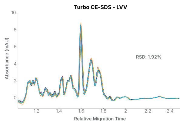
FIGURE 8. Intra-assay reproducibility of the Turbo CE-SDS cartridge analyzing LVV samples. Profiles of nine sample injections from three different preparations demonstrate high reproducibility of the method, with an RSD value of 1.92% for the total area.
