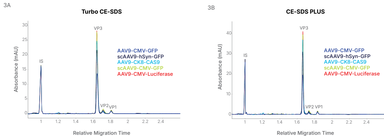
FIGURE 3. Measuring the capsid protein ratio of AAVs with Maurice CE-SDS. Five AAV samples with different transgenes were analyzed with A. Turbo CE-SDS and B. CE-SDS PLUS. Different sample profiles are clearly captured by both methods, from which the respective capsid protein ratios were measured.
