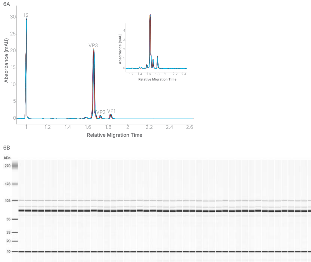
FIGURE 6. Method reproducibility of the CE-SDS PLUS assay. A. Overlaid profiles of 45 AAV sample injections demonstrate the high reproducibility of the method. B. Gel-like view of the same results.
