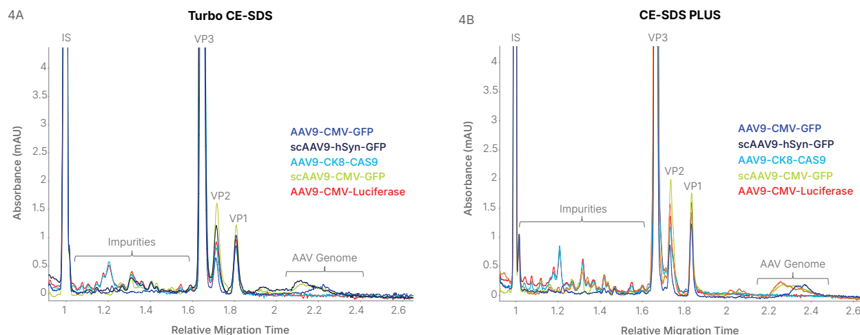
FIGURE 4. Measuring impurities in different AAV samples with Maurice CE-SDS. Five AAV samples with different inserts were analyzed with A. Turbo CE-SDS and B. CE-SDS PLUS. Both methods were able to detect and quantitate the level of impurities and the AAV genome present in the samples.
